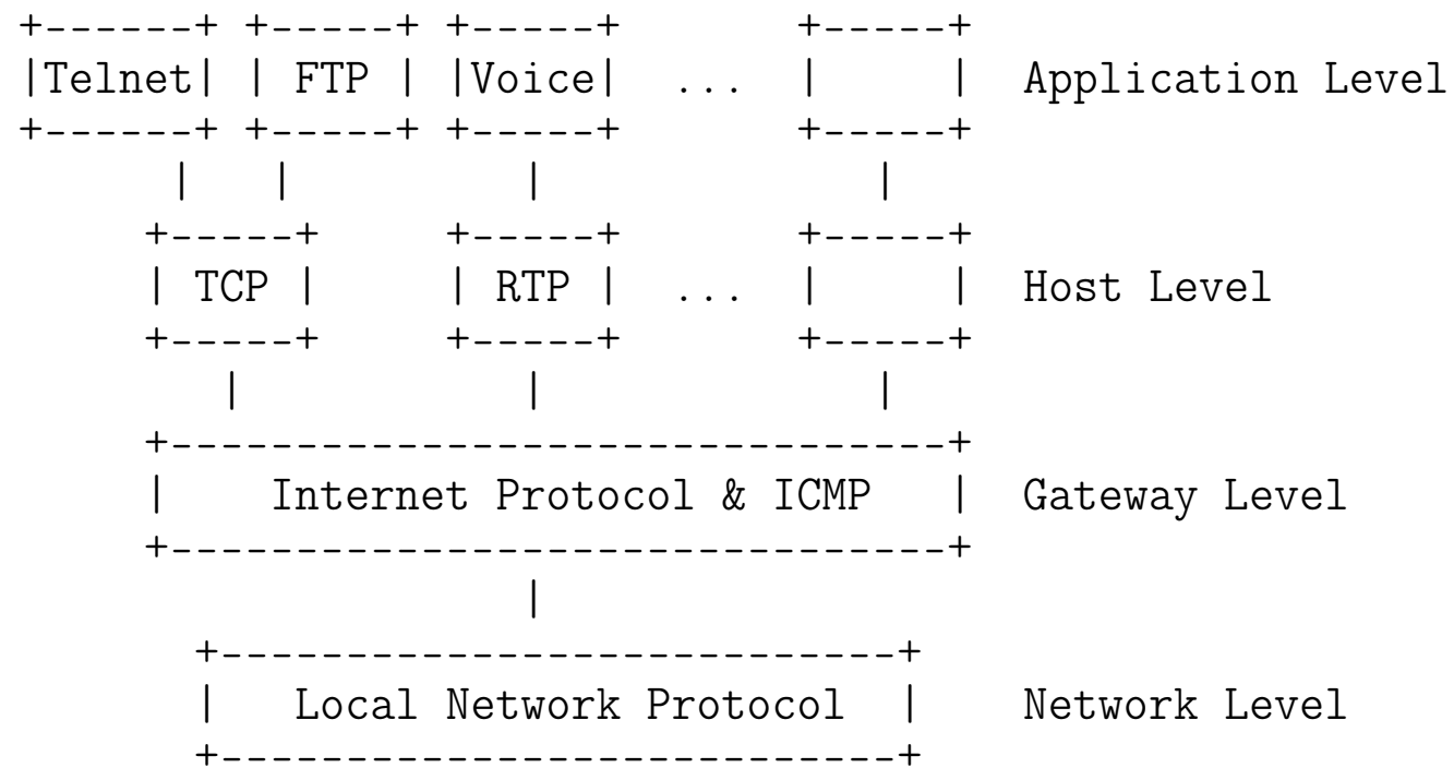
Protocol Relationships
