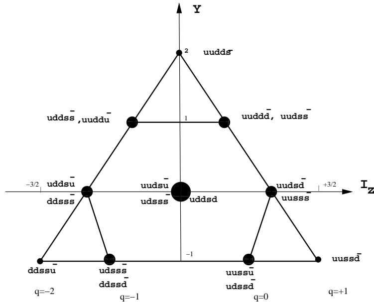
Figure 2. The octet + antidecuplet
