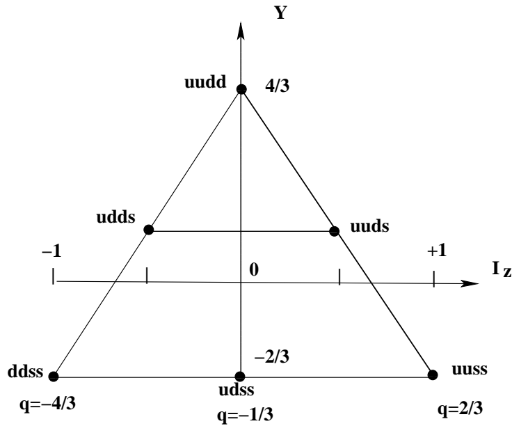
Figure 1. The \{2^2\}^{fl} sextet
